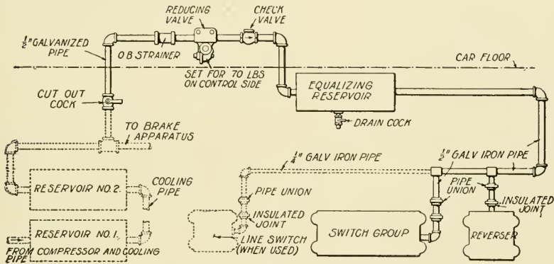
Fig. 73. Piping Diagram, Westinghouse Multiple-Unit System
